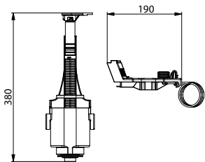
Technical drawing
