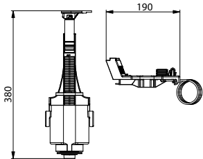
Technical drawing
