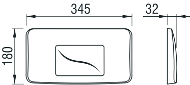
Technical drawing
