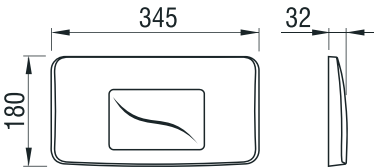
Technical drawing
